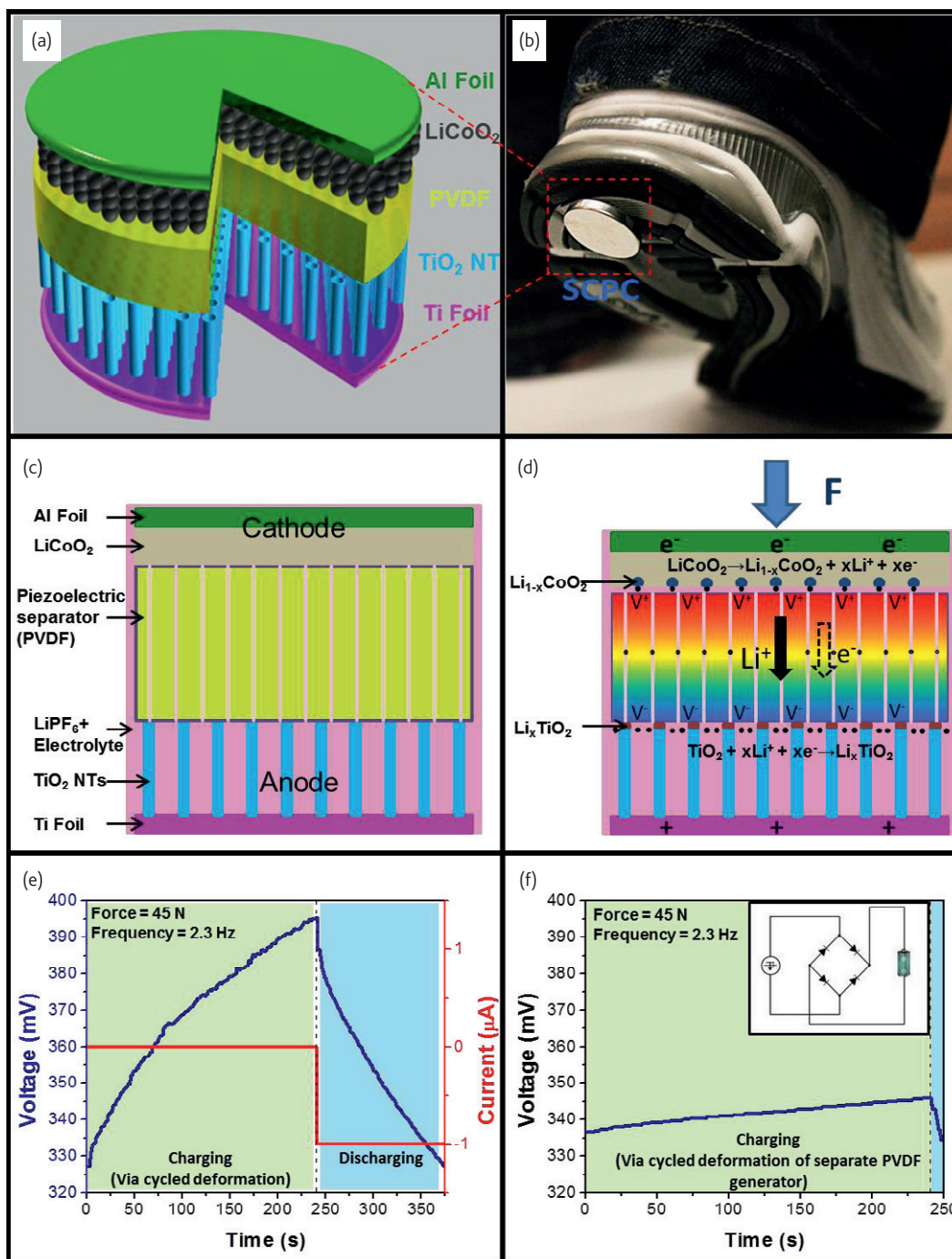
Fig. 8 A self-charging power cell (SCPC) that hybridizes a piezoelectric nanogenerator and a Li-ion battery. (a) Schematic diagram showing the design and structure of the SCPC. The anode is aligned \text{TiO}_2 nanotube arrays that are directly grown on Ti foils; a layer of polarized PVDF film performs as the separator; the cathode is \text{LiCoO}_2 mixture on aluminum foil. (b) Sticking a power cell on the bottom of a shoe, the compressive energy generated by walking can be converted and stored directly by SCPC. (c) & (d) The brief working mechanism of the SCPC driven by compressive straining: (c) schematic illustration of the SCPC in discharged state with \text{LiCoO}_2 as cathode and \text{TiO}_2 nanotubes as anode; (d) under the driving of the piezoelectric field from straining, the Li ions from the cathode will migrate through the PVDF film separator in the electrolyte toward the anode, leading to the corresponding charging reactions at the two electrodes. The free electrons at the cathode and positive charges at the anode will dissipate inside the device system. (e) A typical self-charging process simply by applying cycled mechanical compressive strain to the device (green shadowed region), during which the voltage keeps raising; in the discharge process (blue shadowed region), the stored power is released in the form of electron flow in the external load. (f) As a comparison of efficiency, the SCPC is separated into two individual units: a PVDF piezoelectric generator and a Li-ion battery by using PE as a separator. The inset is a schematic circuit of the traditional charging methods with separated generator and storage units connected by a bridge rectifier (with permission from the America Chemical Society).
