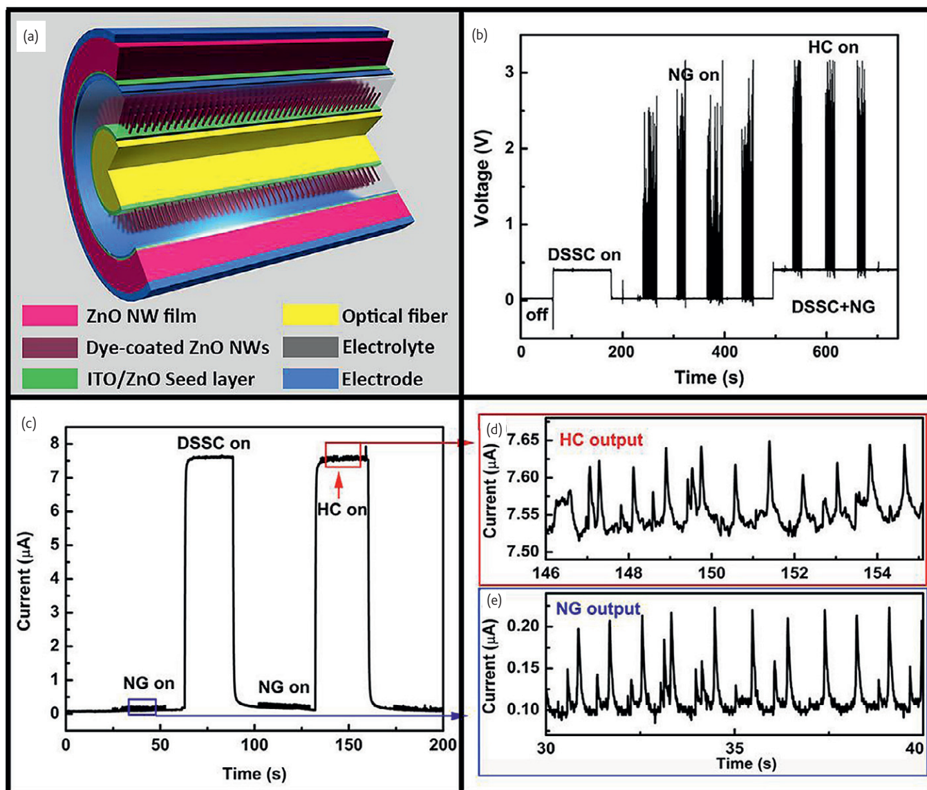
Fig. 6. Design and performance of a 3D optical fiber based hybrid cell (HC) consisting of a dye-sensitized solar cell (DSSC) and a nanogenerator (NG) for harvesting solar and mechanical energy. (a) The 3D HC is composed of an optical fiber based DSSC with capillary tube as counter electrode and a NG on top. (b) Open-circuit voltage ( V_{oc} ) of the HC when the NG and the DSSC are connected in series, where V_{oc(HC)} = V_{oc(DSSC)} + V_{oc(NG)} . (c) Short-circuit current ( I_{sc} ) of the HC when the NG and the DSSC are connected in parallel. (d) and (e) Enlarged view of I_{sc(HC)} and I_{sc(NG)} clearly showing that I_{sc(NG)} is 0.13 \mu\text{A} , the I_{sc(DSSC)} is 7.52 \mu\text{A} , and the I_{sc(HC)} is about 7.65 \mu\text{A} , nearly the sum of the output of the DSSC and the (with permission from Wiley).
