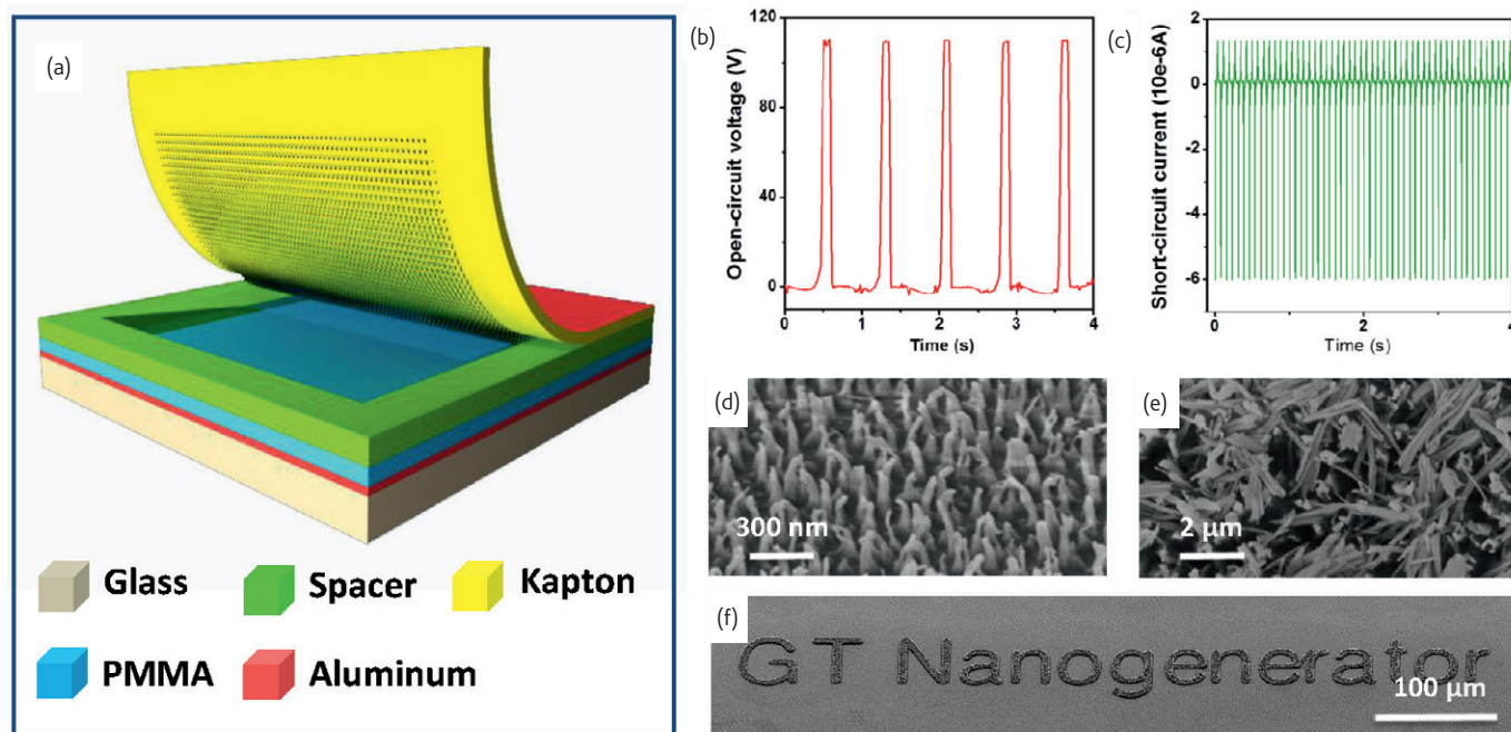
Fig. 3 A design and performance of a triboelectric nanogenerator. (a) A schematic of the miniaturized triboelectric NG. (b) Open-circuit voltage. (c) Short-circuit current. (d) SEM image of polymer NWs on Kapton surface with proper length, showing retained orientation after 1000 times of contacts. (e) SEM image of overly long NWs that have permanent deformation after 1000 contacts. (f) Silver deposits on gold as a result of pulse electrodeposition powered by the triboelectric NG (with permission from America Chemical Society).
