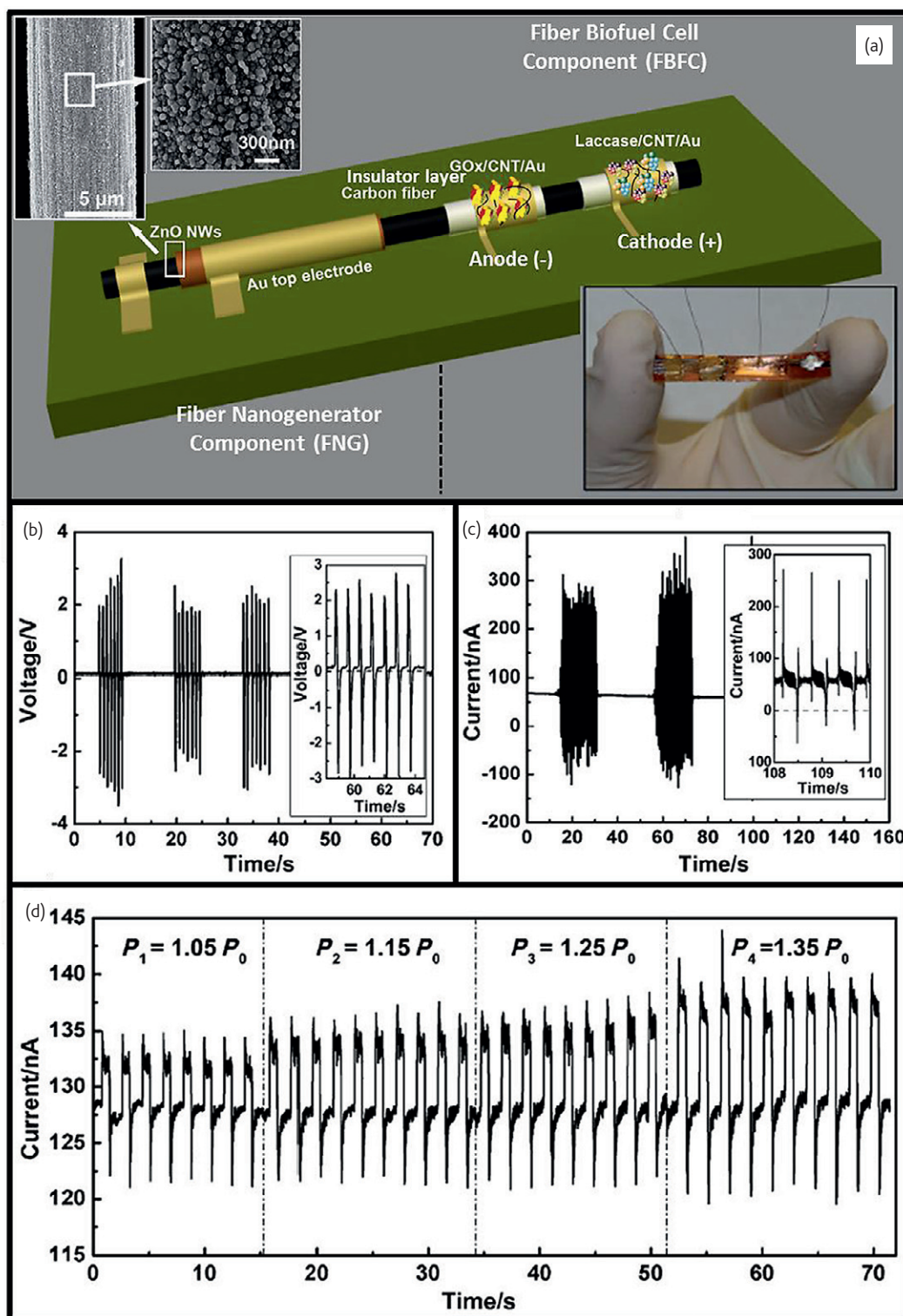
Fig. 7 Design and electrical measurement of a single fiber-based HC for simultaneously harvesting of biochemical and biomechanical energies from an external force or pressure applied to a liquid. (a) Schematic 3D representation of the HC. The insets in the upper left are SEM images of a textured ZnO NW film grown around a carbon fiber composed of densely packed ZnO NW. A digital picture of the device is shown at the lower corner. (b) Open-circuit voltage of the HC when the FNG and the FBFC are connected in parallel. (c) Short-circuit current of the HC when the FNG and the FBFC are connected in series. The insets in (b) and (c) are enlarged plots of the corresponding outputs showing the details of the signals; dashed lines indicated the zero-output line. (d) Response of the HC system to periodically applied pressure (with permission from Wiley).
