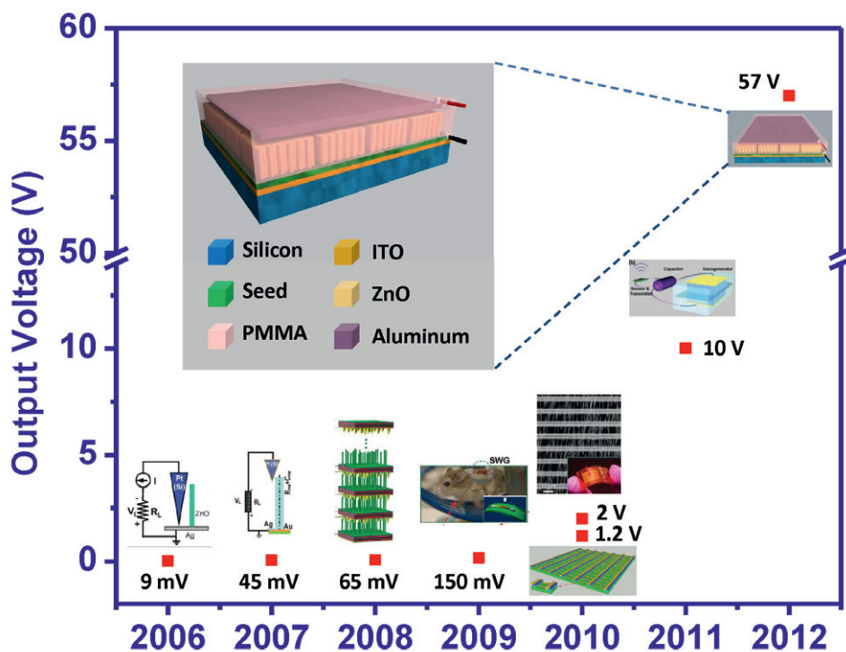
Fig. 1 A summary on the development of high output piezoelectric nanogenerators ever since it was invented in 2006. Inset: the schematic of the mostly recently developed integrated nanogenerator based on vertically aligned ZnO arrays.
